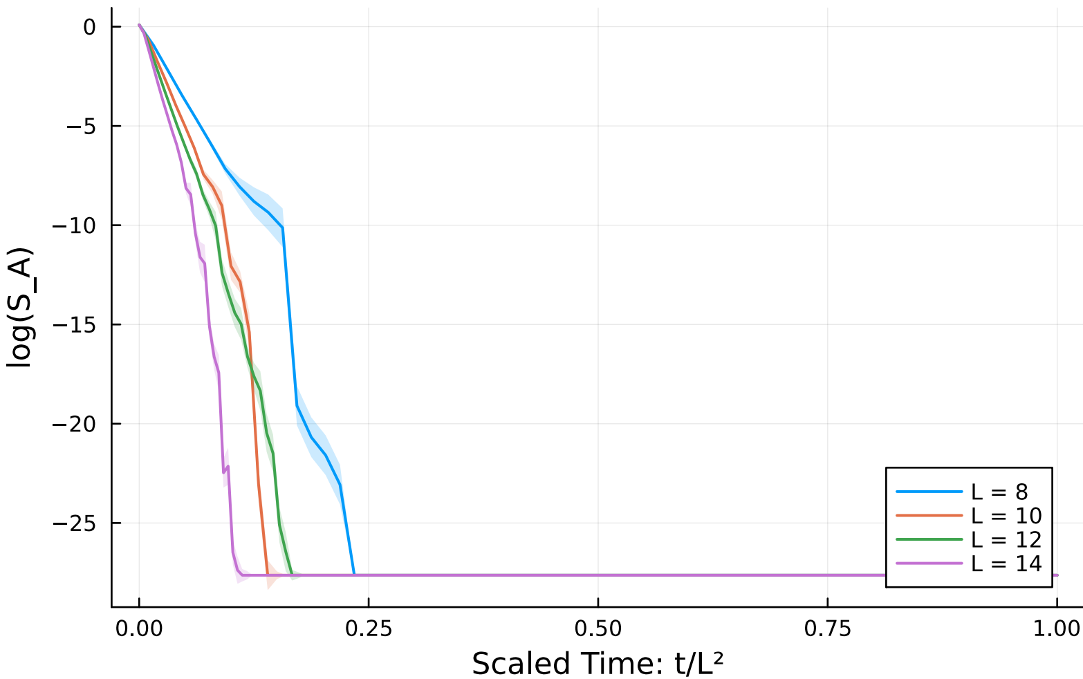
Scaled Log Entropy Evolution ( p = 0.800000 )
